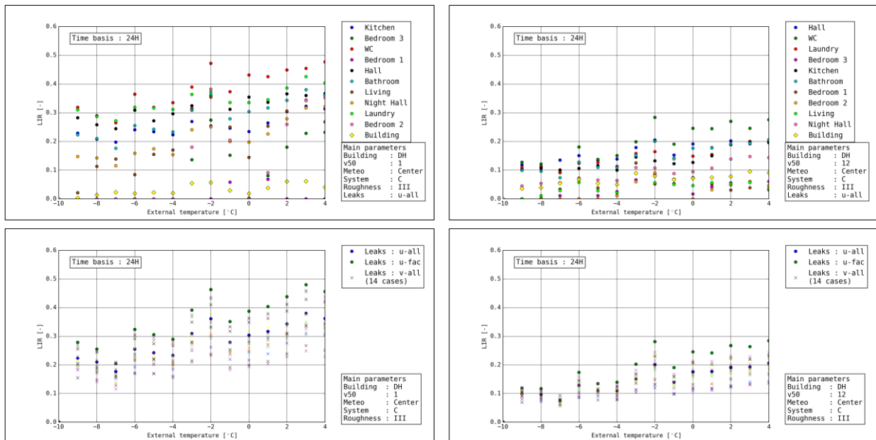
Figure 5 Upper left: LIR per room with good airtightness ( v_{50}=1 ); Upper right: LIR per room with bad airtightness ( v_{50}=12 ); Lower left: sensitivity to leak's distribution for bathroom ( v_{50}=1 ); Lower right: sensitivity to leak's distribution for bathroom ( v_{50}=12 )
