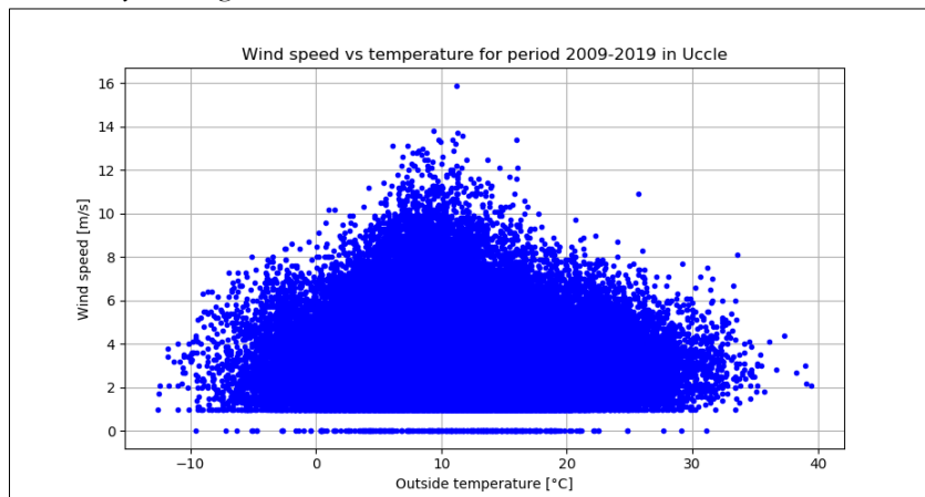
Figure 1 Wind speed versus outside temperature from the period 08/2009 to 07/2019 in the Uccle (Brussels) Royal Meteorological Institute weather station – hourly data
