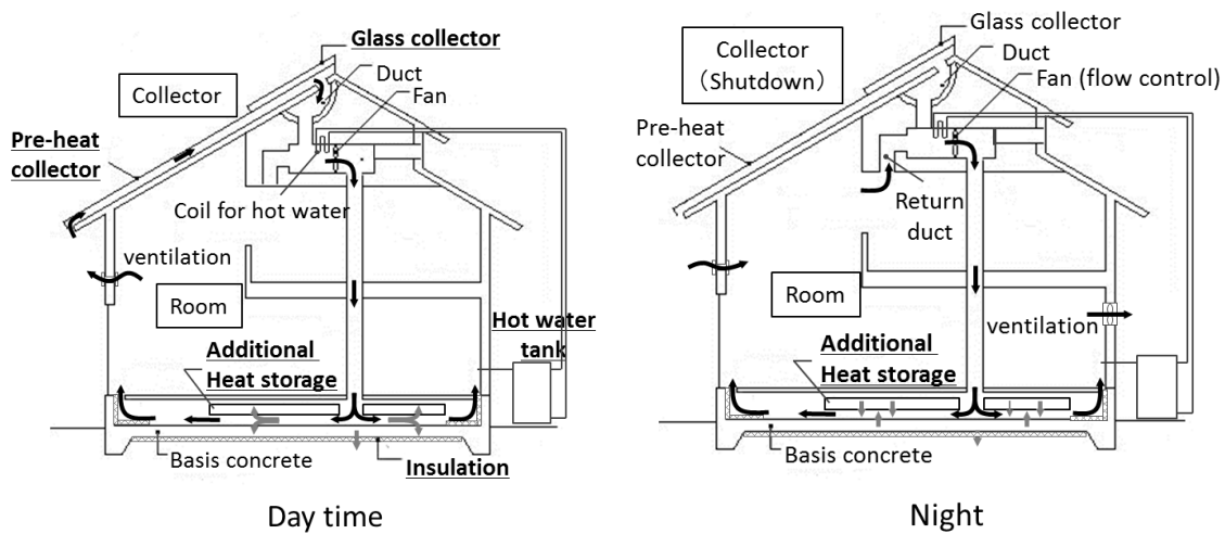
Figure 3: Heat balance of air-based solar system
