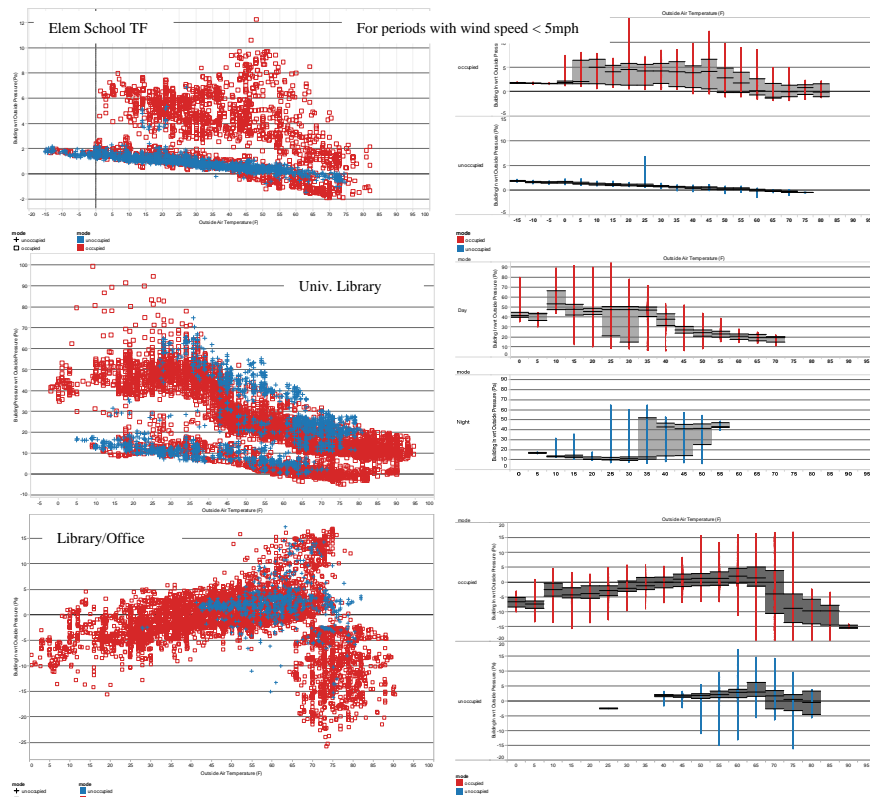
Figure 5: Occupied and unoccupied mode building pressure with outside temperature
