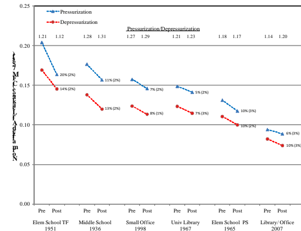
Figure 1: Building normalized envelope leakage pre and post air sealing
