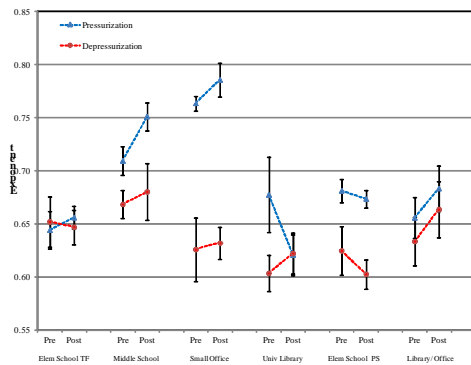
Figure 3: Power law flow equation exponent pre and post air sealing
