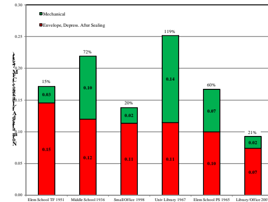
Figure 4: Building normalized envelope and mechanical system leakage
