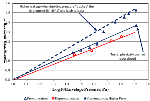
Figure 2: Pressurization and depressurization leakage tests on a door with a loose latch
