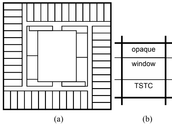
Figure 1 (a) Floor plan and (b) façade layout of one cell office with an opaque area, a window in the visual area and transparent solar thermal collectors (TSTC) in the spandrel area.
