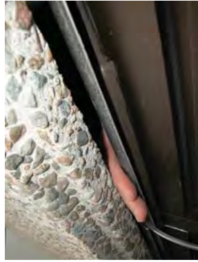
Figure 13: Dismantlement of interior finishes at window head reveals direct air leakage path.
