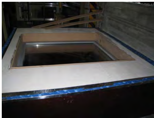
Figure 2a, calibration setup for measuring extraneous air leakage of the setup. Figure 2b, Installation of aluminum window frame and wood reveal.
