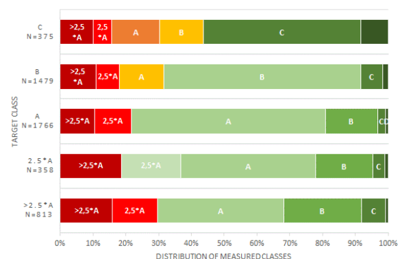
Figure 7: Distribution of ductwork airtightness measured classes depending on target classes - Source: Bassam Moujalled, BEPOSTIVE 2021, Lyon, France, December 2021.
