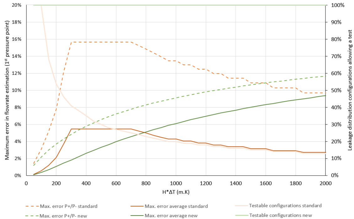
Figure 5: Maximum error and percentage of testable configurations according to the product H \cdot \Delta T ; both according to the standard and new criteria [5]
