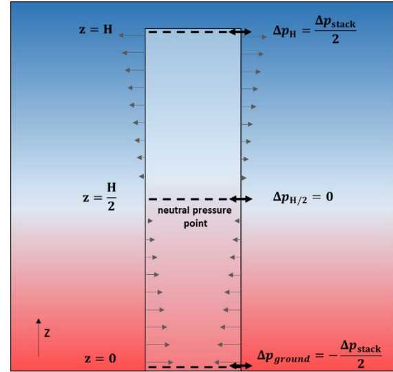
Figure 3: Stack effect in case of evenly distributed leakages along the building's height
