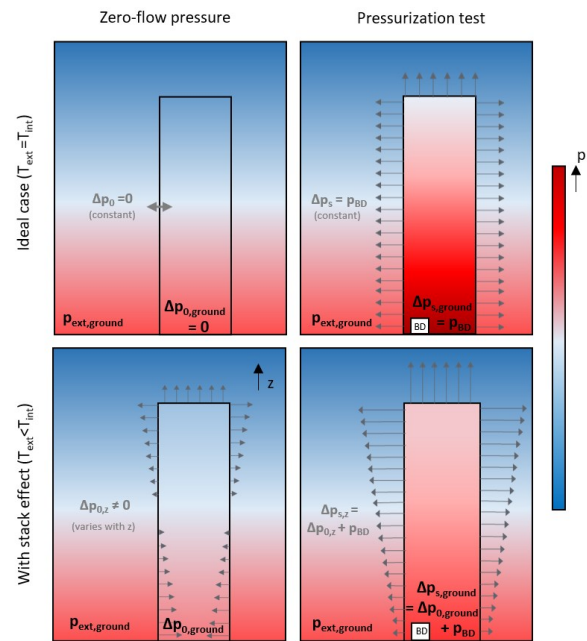
Figure 1: Impact of stack effect for pressurization tests on high-rise buildings
