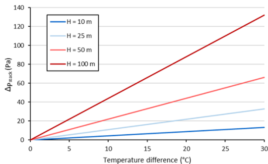
Figure 2: Variation of pressure difference (stack effect only) between the top and the bottom of a building depending on its height and the temperature difference between inside and outside
