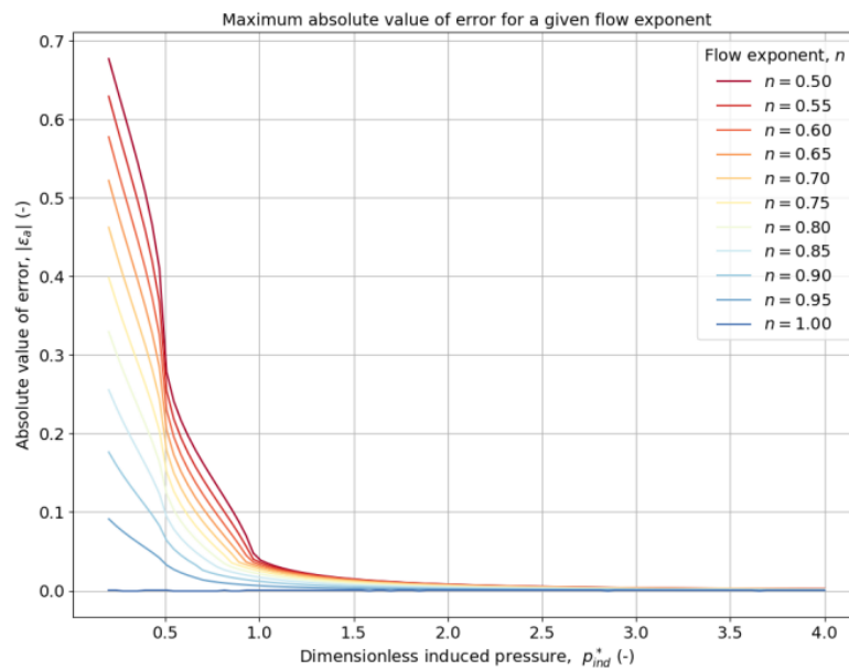
Figure 6: Maximum absolute value of the error as a function of dimensionless induced pressure error for various flow exponents. Averaging pressurization and depressurization tests.[2]
