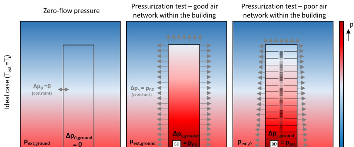
Figure 4: Impact of obstacles for pressurization tests on high-rise buildings (Obstacles for the flow can generate poor air network within a leaky building)
