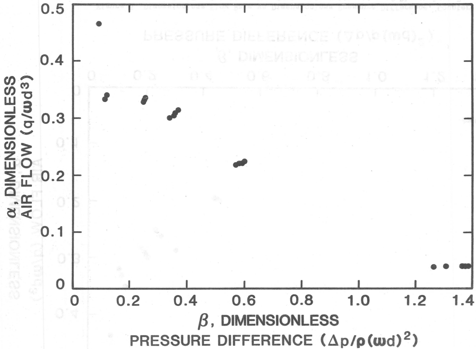
Figure 6 Dimensionless Flow Rate vs Dimensionless Pressure Difference, Clockwise Fan Rotation, Manufacturer's Calibration of Blower Door B
