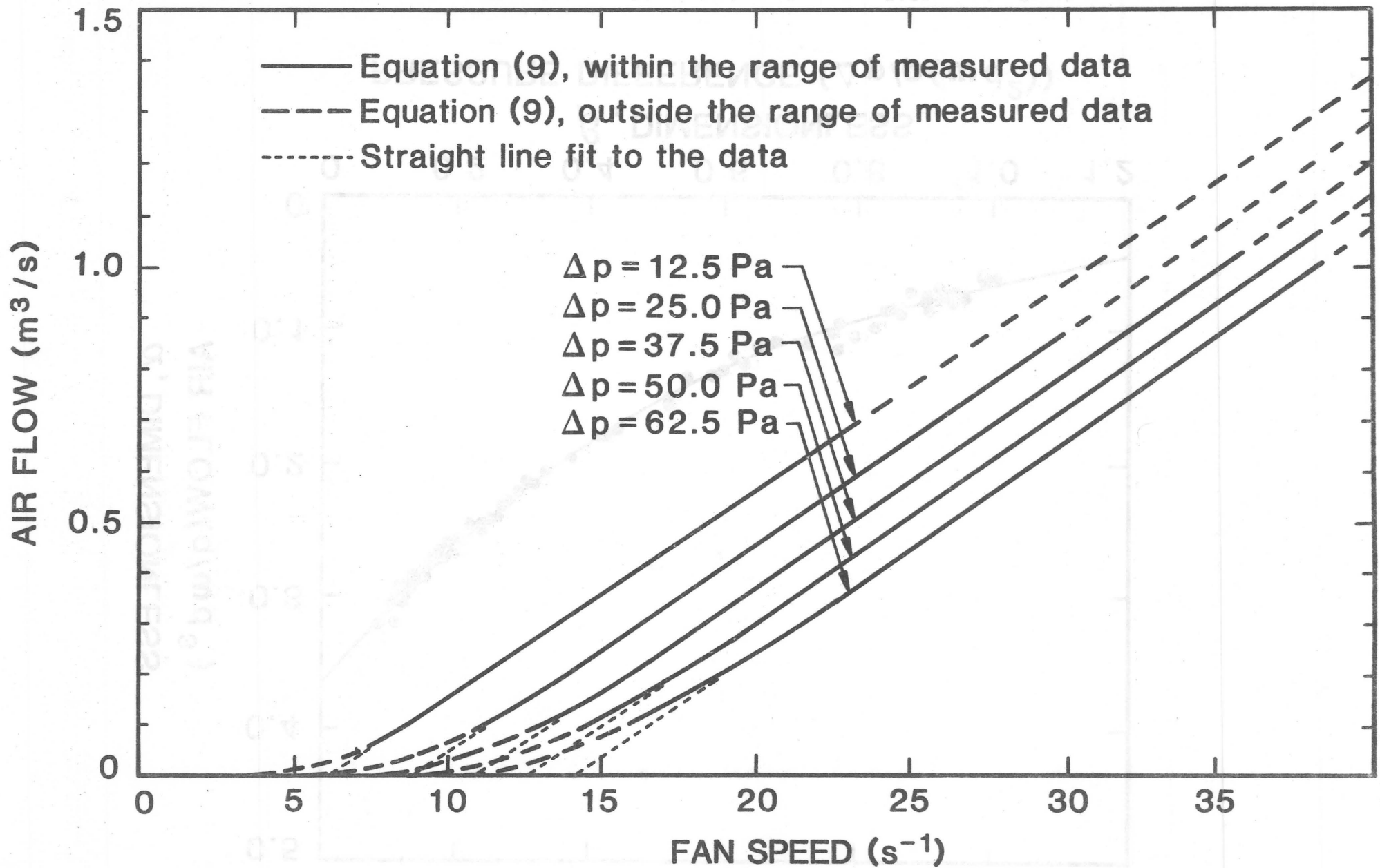
Figure 4 Air Flow Rate vs Fan Speed at Several Pressure Differences
