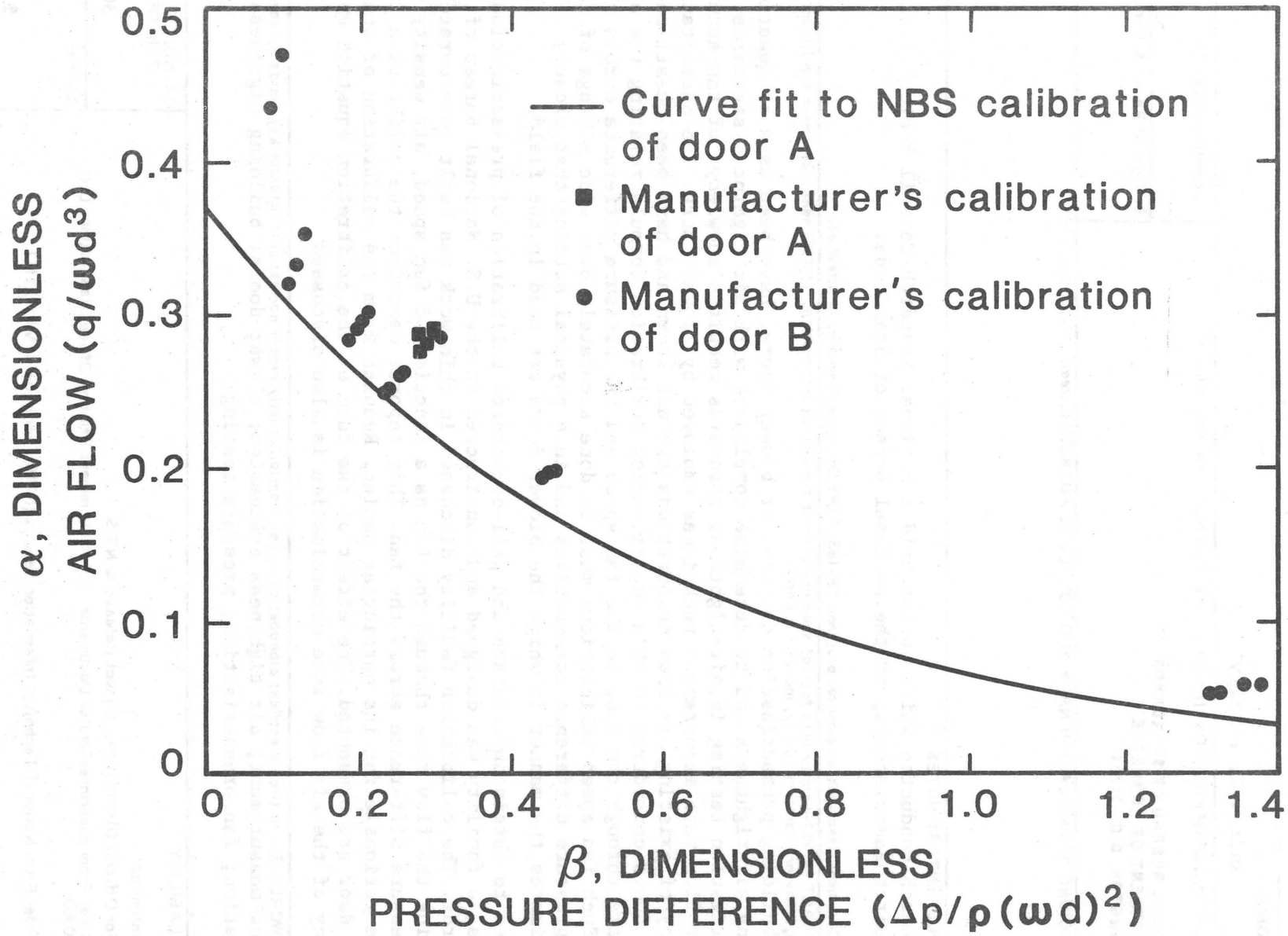
Figure 7 Comparison of Calibrations of Blower Doors A and B
