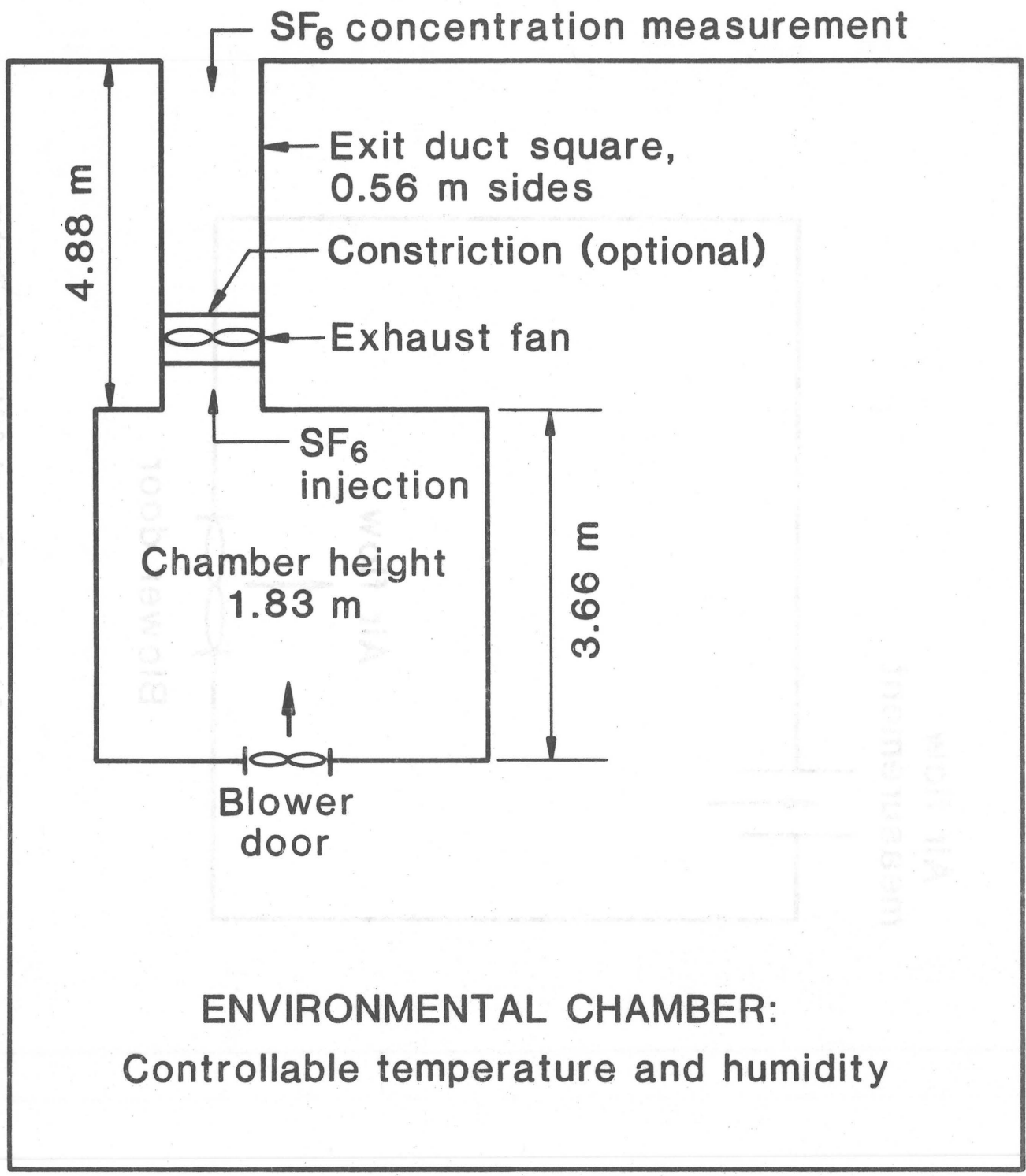
Figure 2 Schematic of NBS Calibration Facility
