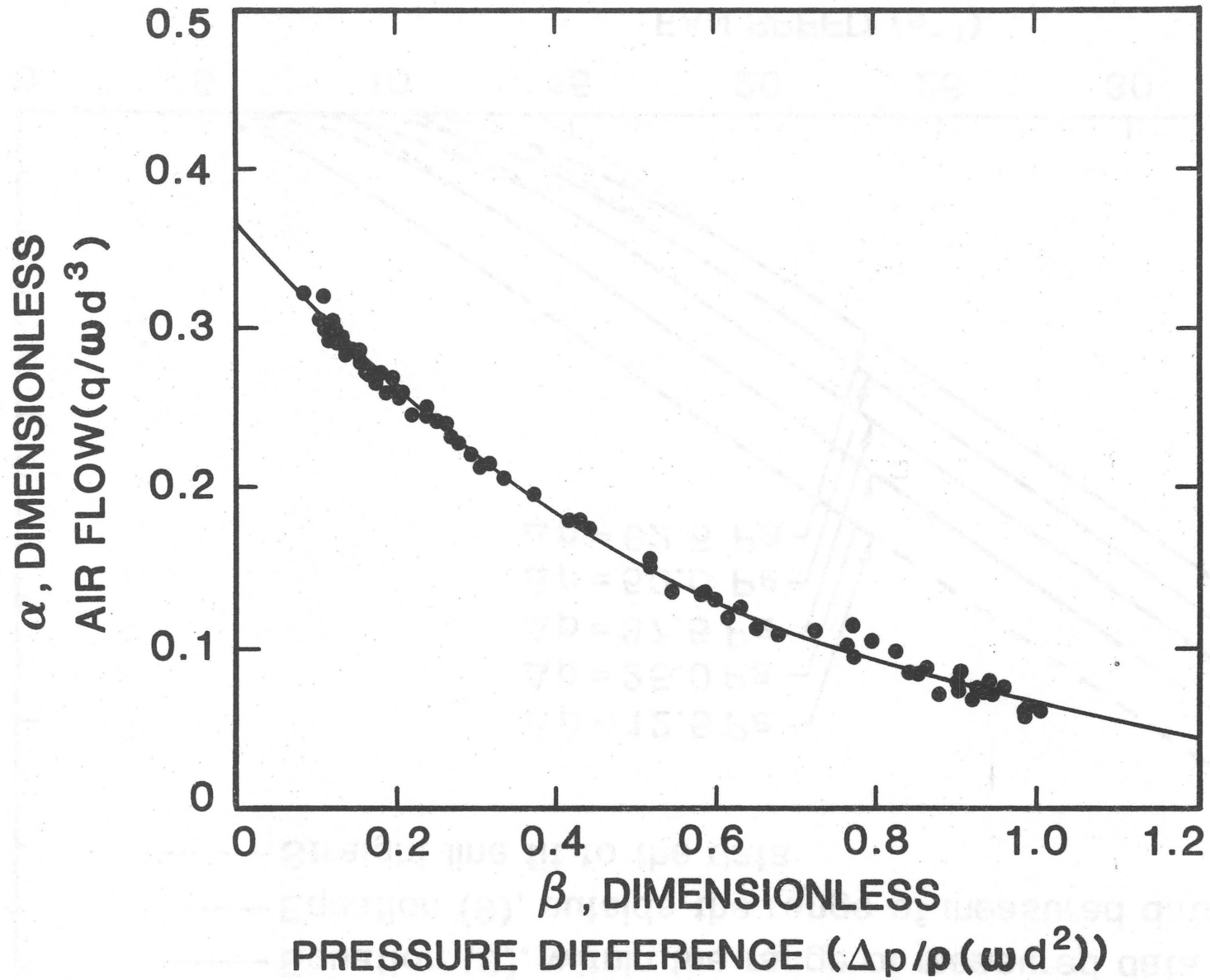
Figure 3 Dimensionless Flow Rate vs Dimensionless Pressure Difference, Counter-Clockwise Fan Rotation, NBS Calibration of Blower Door A
