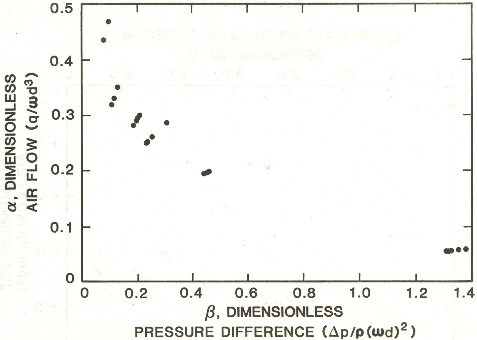
Figure 5 Dimensionless Flow Rate vs Dimensionless Pressure Difference, Counter-Clockwise Fan Rotation, Manufacturer's Calibration of Blower Door B
