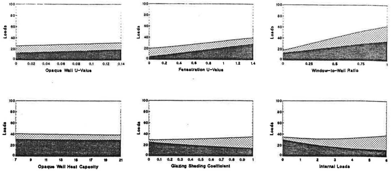
Figure 5. Loads vs. Envelope Parameters for Seattle, Washington
