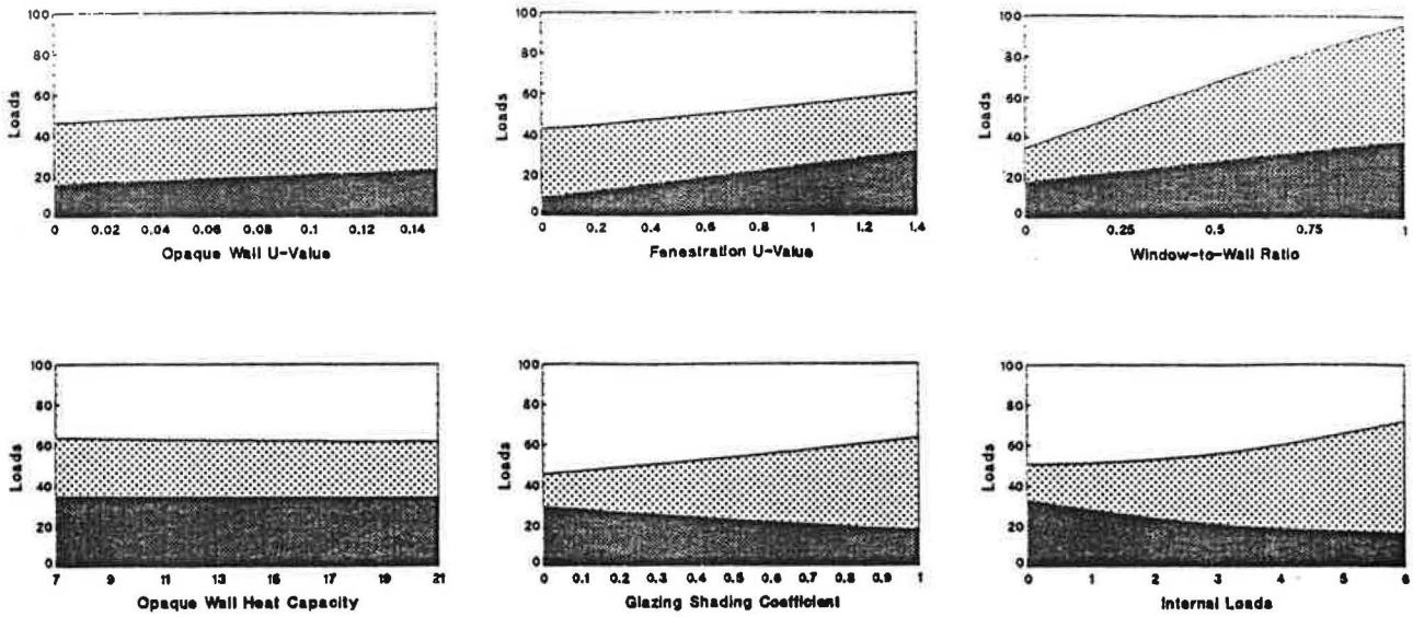
Figure 1. Loads vs. Envelope Parameters for Washington, DC
