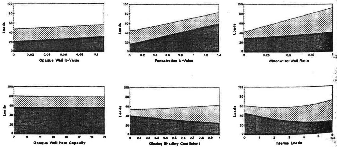
Figure 6. Loads vs. Envelope Parameters for Minneapolis, Minnesota
