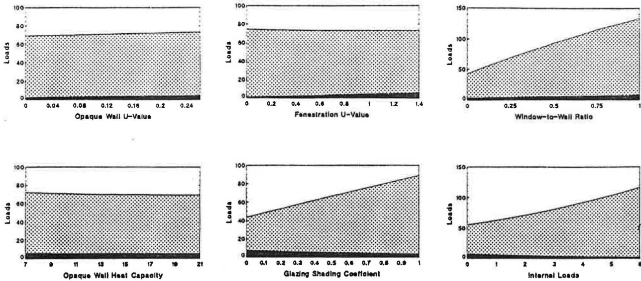
Figure 3. Loads vs. Envelope Parameters for Houston, Texas
