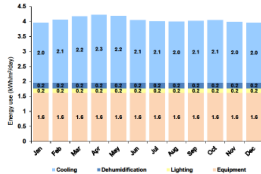
Figure 10: Energy used in passive and air-conditioned alternatives.
