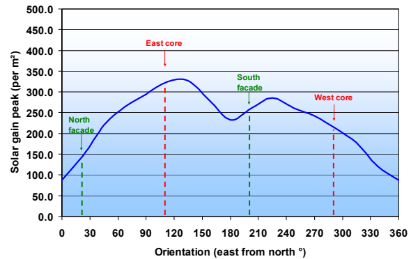
Figure 1: Solar gain by orientation.
