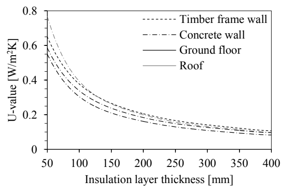
Figure 1 The building envelope U-values as a function of insulation thickness
